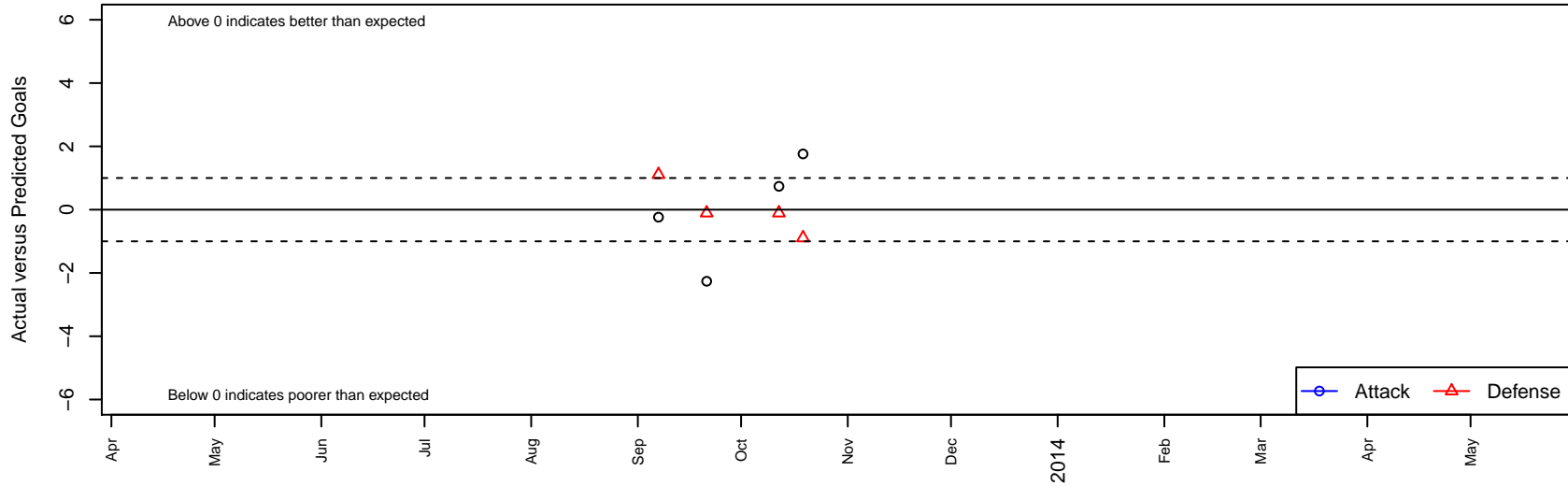
California Northstars B01 Dots are actual minus expected GF (blue circles) and GA (red triangles). Blue line is smoothed change in attack strength. Red is smoothed change in defense strength.
